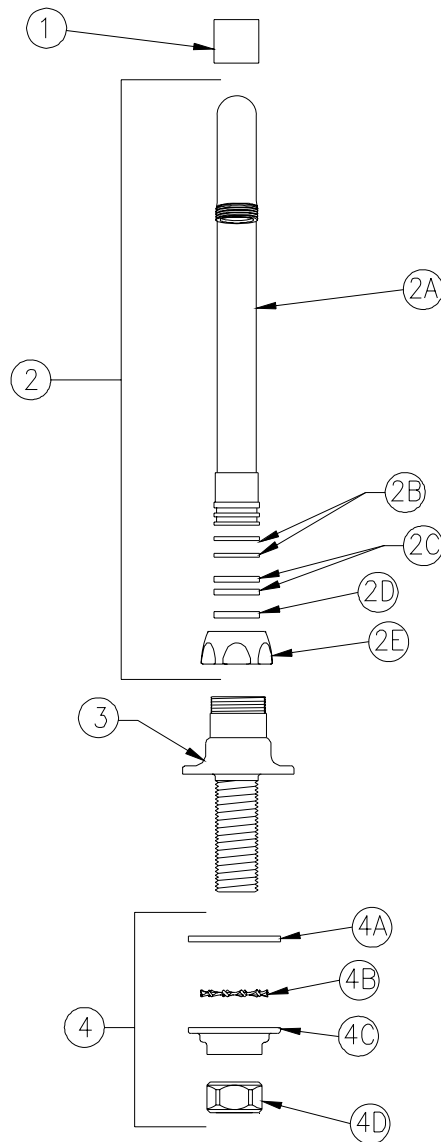
Z821B0 SHOWN
